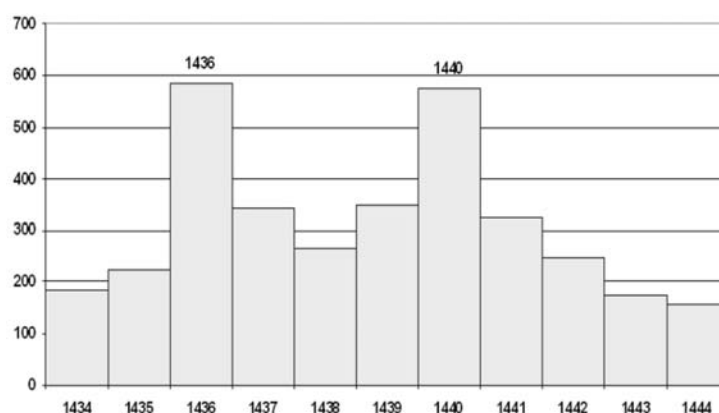
Figure 4: a) Example of Near Zone Effect and daily period [6], b) splitting of daily period on solar and star periods [7]. X-axis – time intervals between pairs of similar histograms, a) – hours, b) – minutes; Y-axis – number of similar histogram pairs found by expert.
