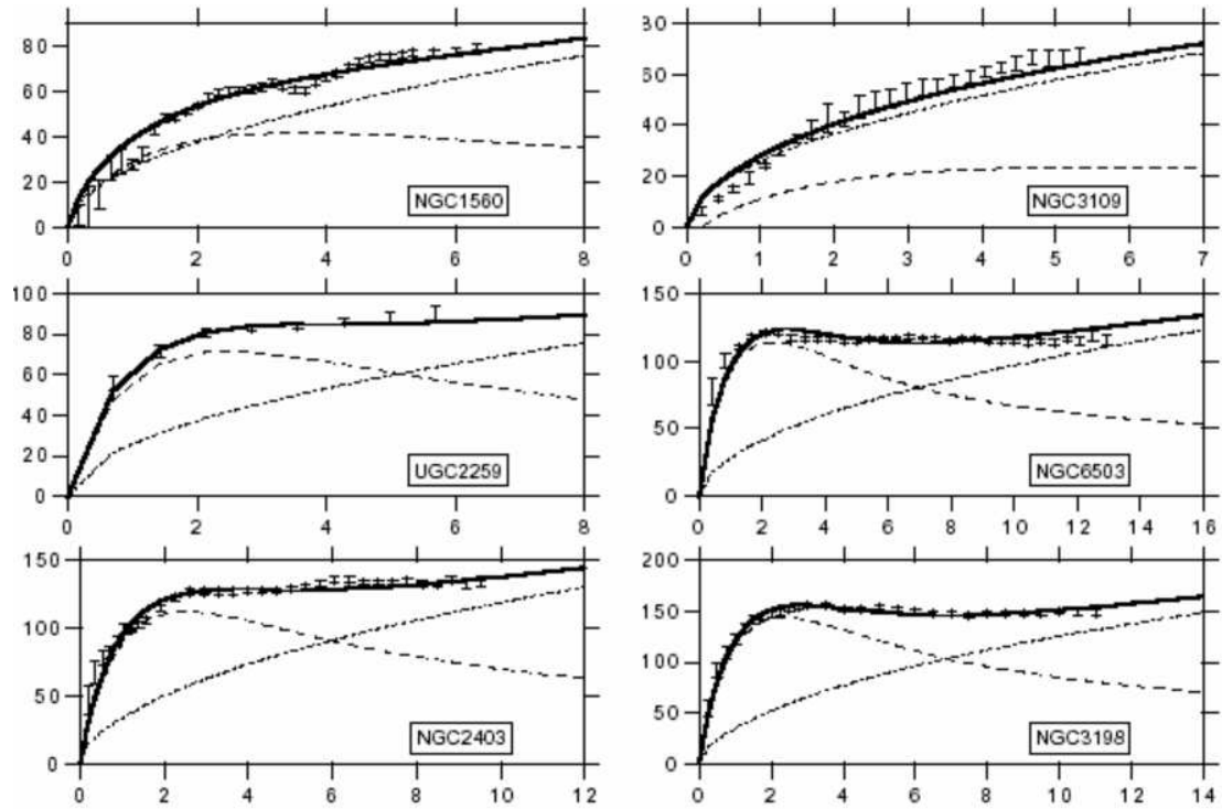
Figure 1: [4] Orbital velocities (km/s) as functions of R/R_0 , where R_0 is a characteristic scale for each galaxy. Dashed line is the Newtonian potential (coinciding with the Schwarzschild's solution), produced by the observable gleaming matter with regard to the exponential distribution of stars inside the galaxy.
