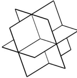
Figure 1: Isotropic planes of tree-dimensional time
