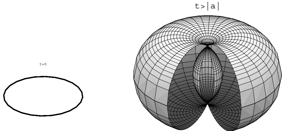
Figure 1: The shape of singular locus for electromagnetic field (8.5) of electrically neutral solution (8.4) at initial ( t = 0 ) and final ( t > |a| ) instants
