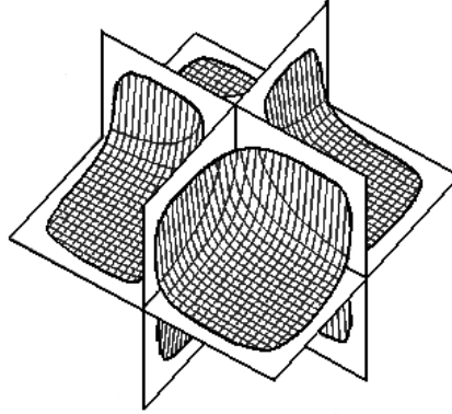
Figure 4: The eight-sheet hyperboloid of tree-dimensional time
