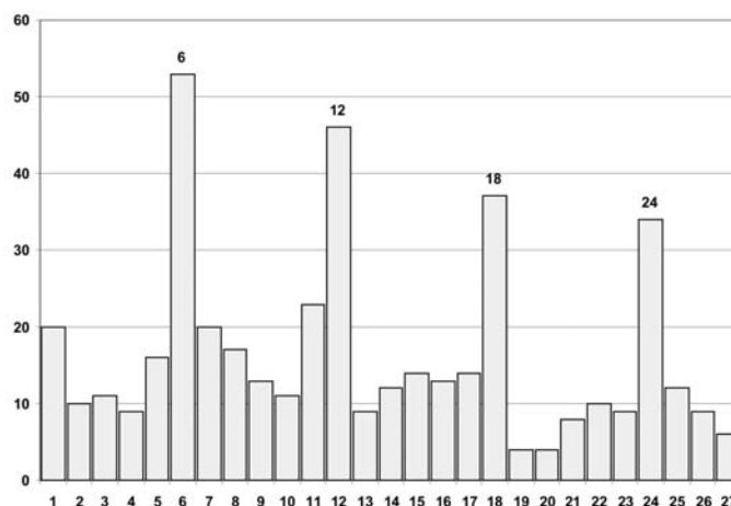
Figure 6: Interval distribution obtained on the base of 60-min histograms constructed from measurements of \alpha -decay rate fluctuations of collimated ^{239}\text{Pu} source.
