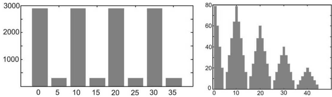
Figure 8: Idealized diagram of rotation speed of centrifuge rotor with time, a ); expected interval distribution, b ).
