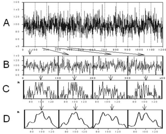
Figure 1: Processing of initial time series. The method of smoothed histograms set obtaining.
