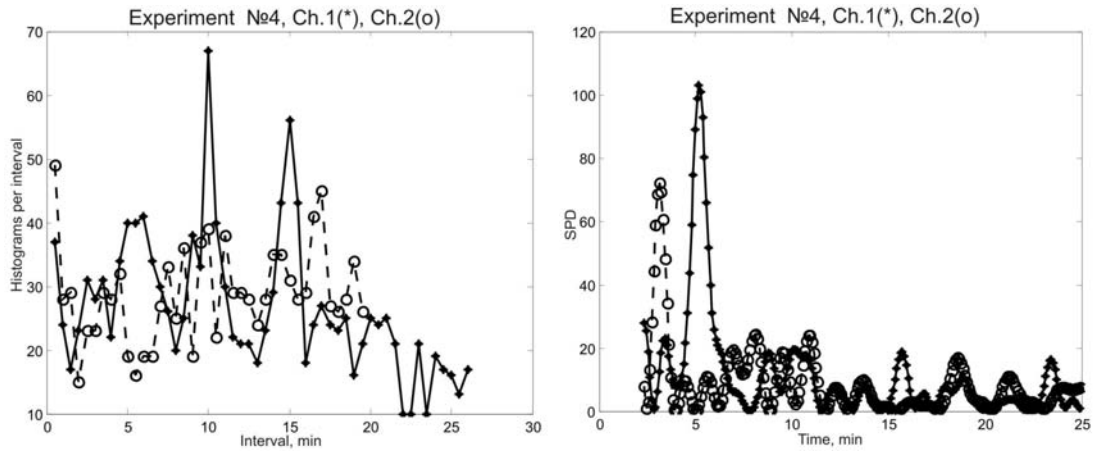
Figure 11: An Example of interval distribution for Ch. 1 (*) and Ch. 2 (°) (series No. 4), a); and corresponding densities of power spectrum, b).
