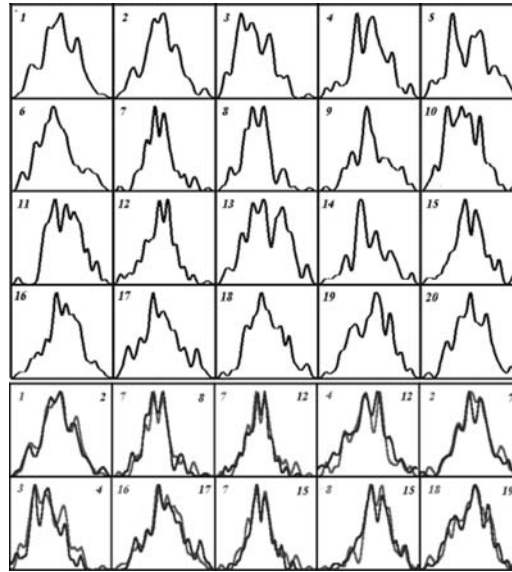
Figure 2: Initial set of smoothed histograms and pairs of similar histograms.
