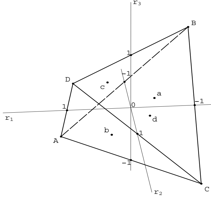
Figure 1: The range of admissible values of r_1 , r_2 and r_3 .
