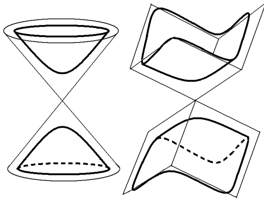
Figure 3: The fragments of unit hyperboloids
