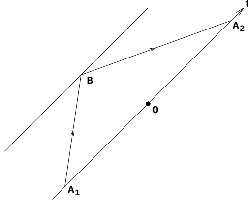
Figure 1: The measuring of a distance between world lines by prelight signals exchange.
