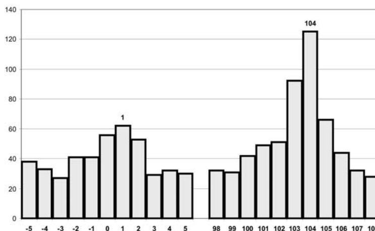
Figure 5: Synchronous changes of histogram's shape similarity in different geographical locations. Left intervals distribution presents the effect of histogram similarity by absolute time, right distribution presents similarity by local time.
