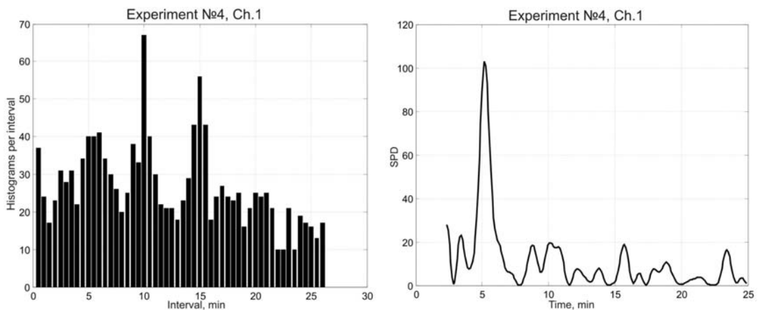
Figure 10: An example of interval distribution (Ch. 1, series No. 4), a ); and corresponding density function of power spectrum, b ).
