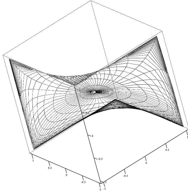
Figure 8: The simultaneous surface of three-dimensional time
