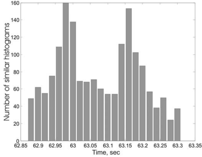
Figure 1: Intervals distributions obtained after expert comparisons of 1-sec (a), 0.2-sec (b), and 0.002-sec (c) histogram sets. Y-axis presents number of histograms, which were found similar; X-axis – time interval between pairs of histograms, sec.
