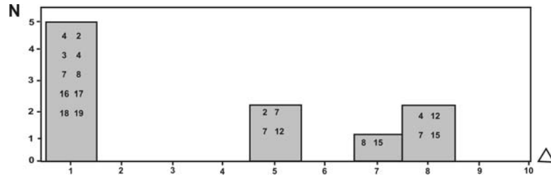
Figure 3: An example of distribution of similar histograms by intervals between them for the set of histograms presented on the fig. 2A.
