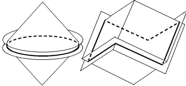
Figure 5: The two light cones couple intersection
