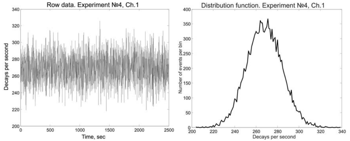
Figure 9: An example of experimental record of \alpha -decay rate fluctuations obtained from ^{239}\text{Pu} -source (Ch. 1, series No. 4), a ; and corresponding distribution function, b .
