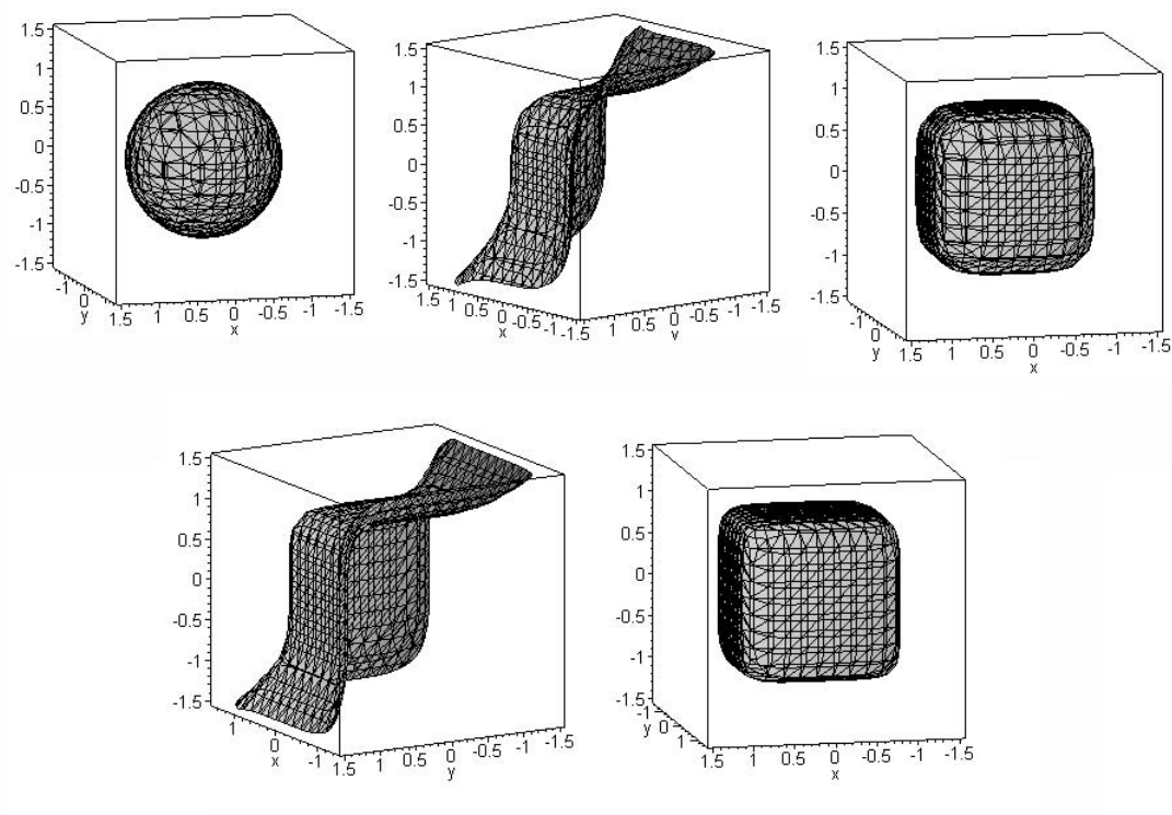
Berwald-Moor indicatrices for k \in \{2, \dots, 6\} ( m = 3 )
