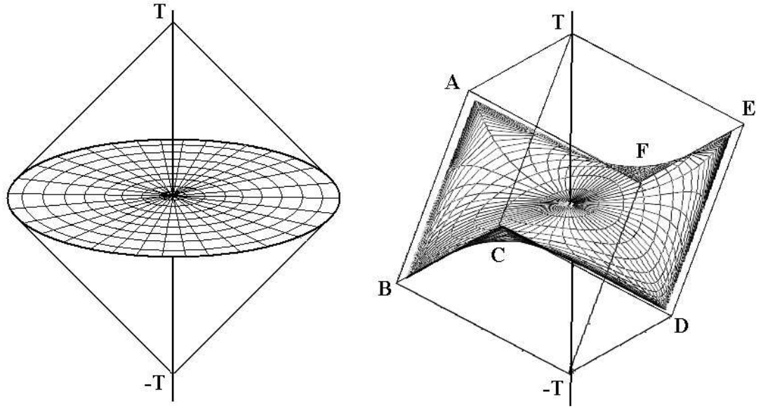
Figure 2: Example of surfaces with dots, equidistant from two fixed dots ( T and -T ) in three-dimensional a) pseudoeuclidean and b) Finsler spaces.
