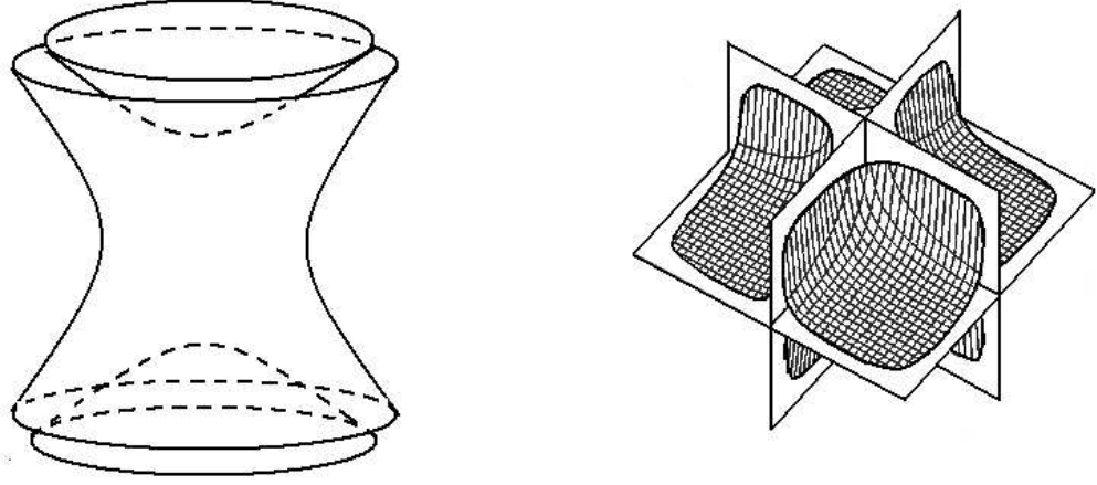
Figure 1: Indicatrix examples in three-dimensional a) pseudoeuclidean and b) Finsler spaces.
